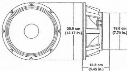
FIGURE 5 — Dimensions
