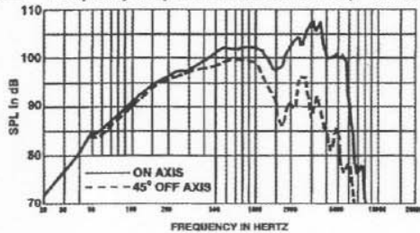
FIGURE 2 — Frequency Response in Standard Baffle (0° and 45°)
