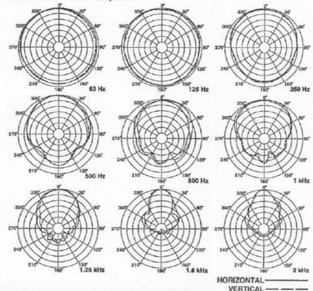
FIGURE 9 — Polar Response
