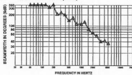
FIGURE 8 — Directivity vs. Frequency
