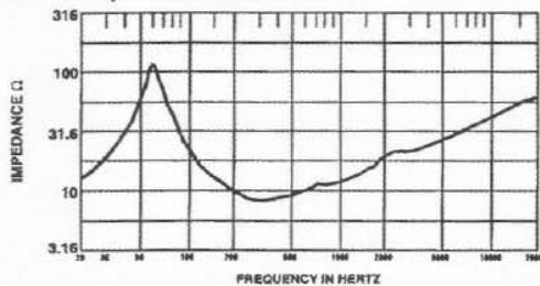
FIGURE 4 — Impedance in Typical Enclosure (2.0 ft 3 )
